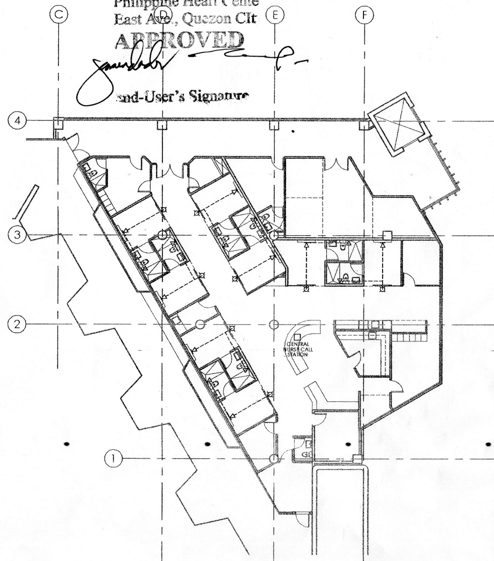
4/F NURSE CALL SYSTEM LAYOUT
