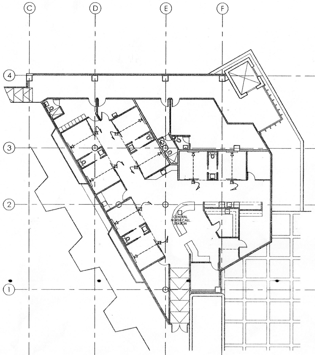
2/F NURSE CALL SYSTEM LAYOUT
